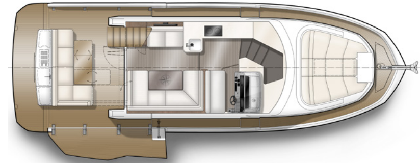
COCKPIT/MAIN DECK
